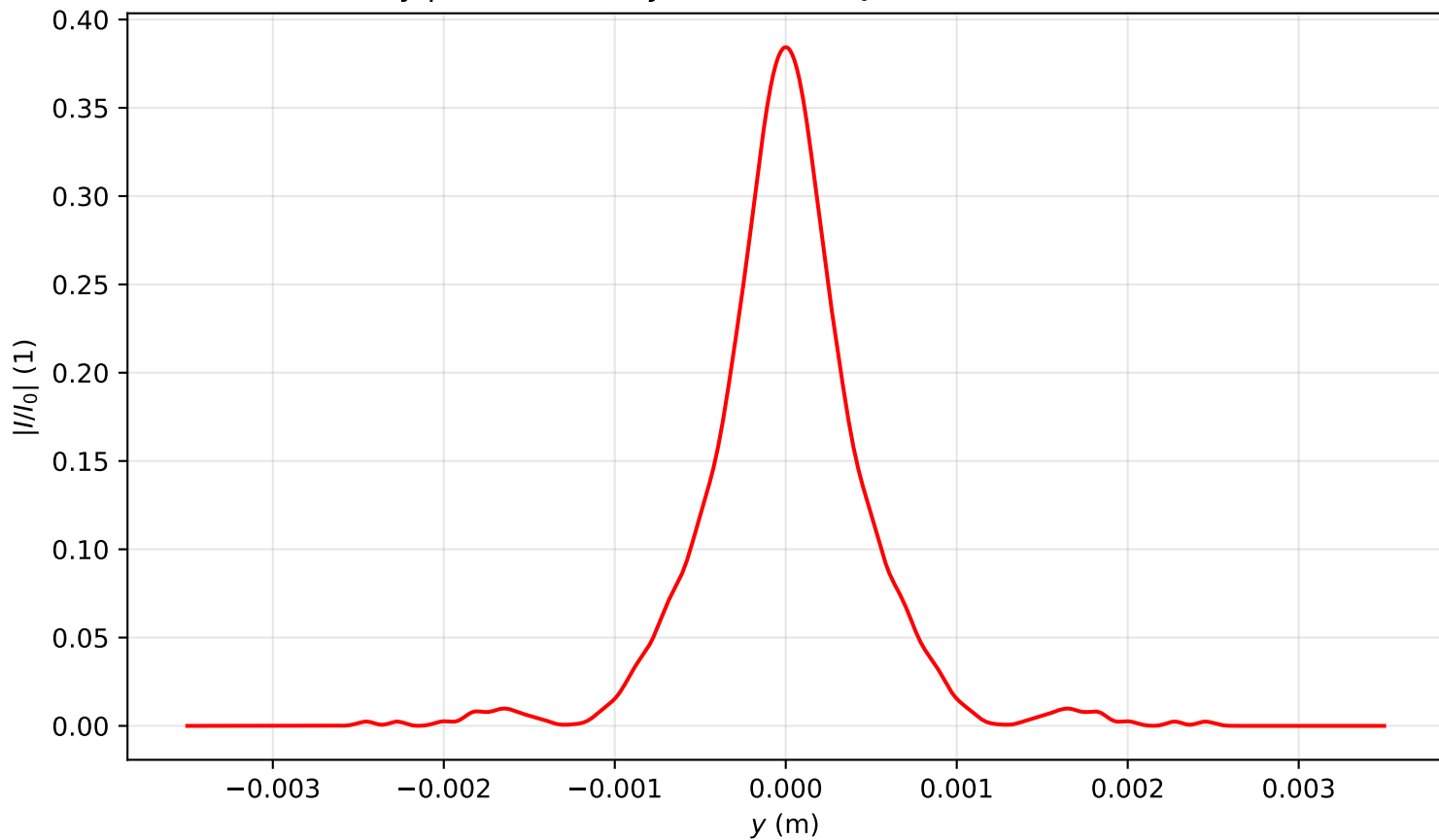
Intensity profile I(x = 0, y, z = 1.274)/I_0 , P_{in}=3.0P_{cr} , artificial time
